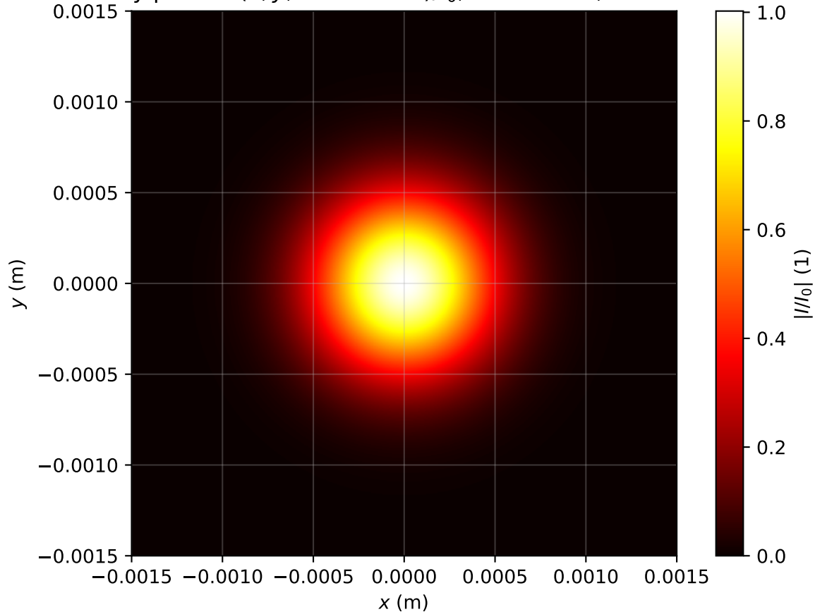
Intensity profile I(x, y, z = 0.080\text{m})/I_0 , \text{Pin}=0.6\text{Pcr} , artificial time
